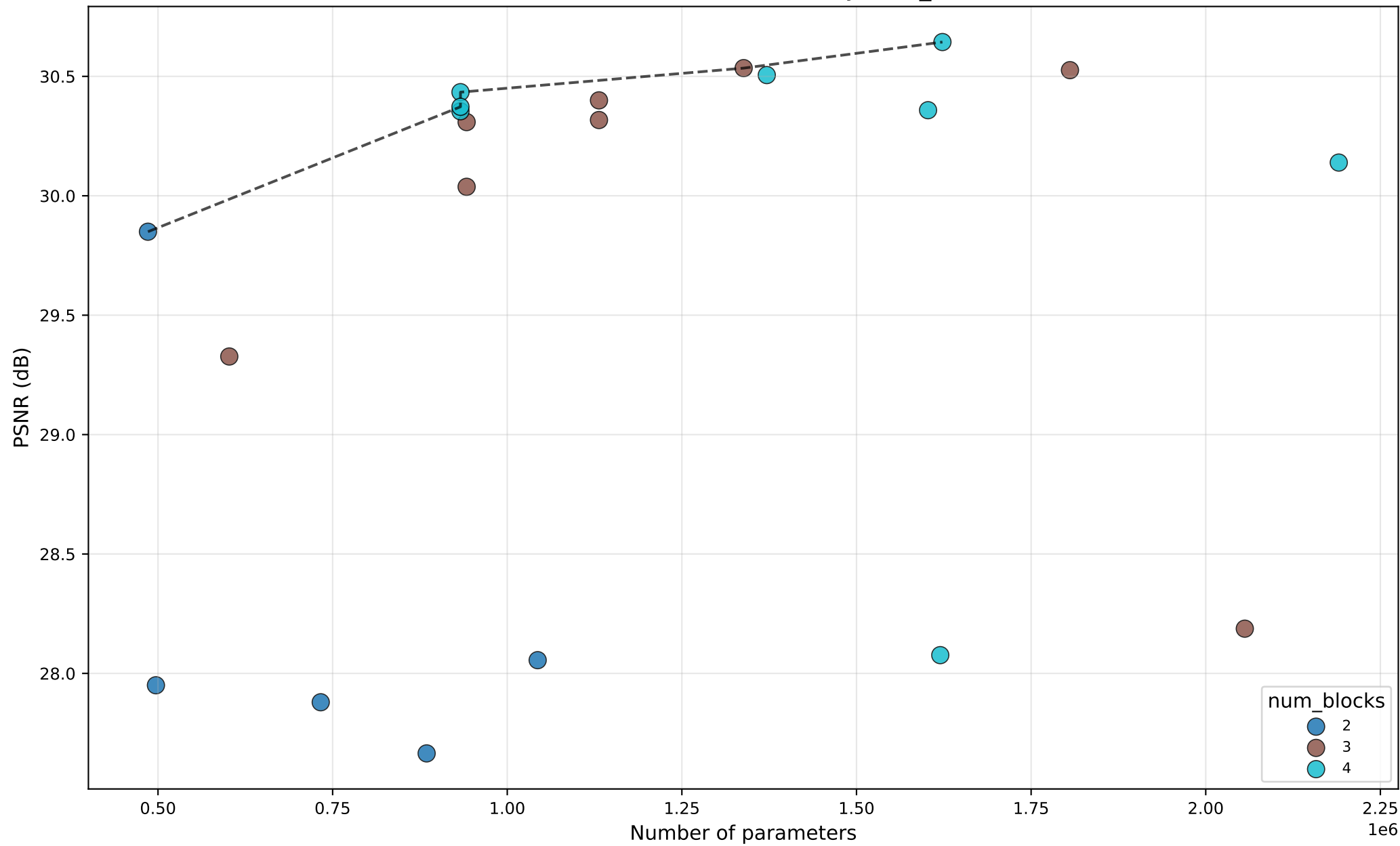
PSNR vs #Params — ELAN — by num_blocks
